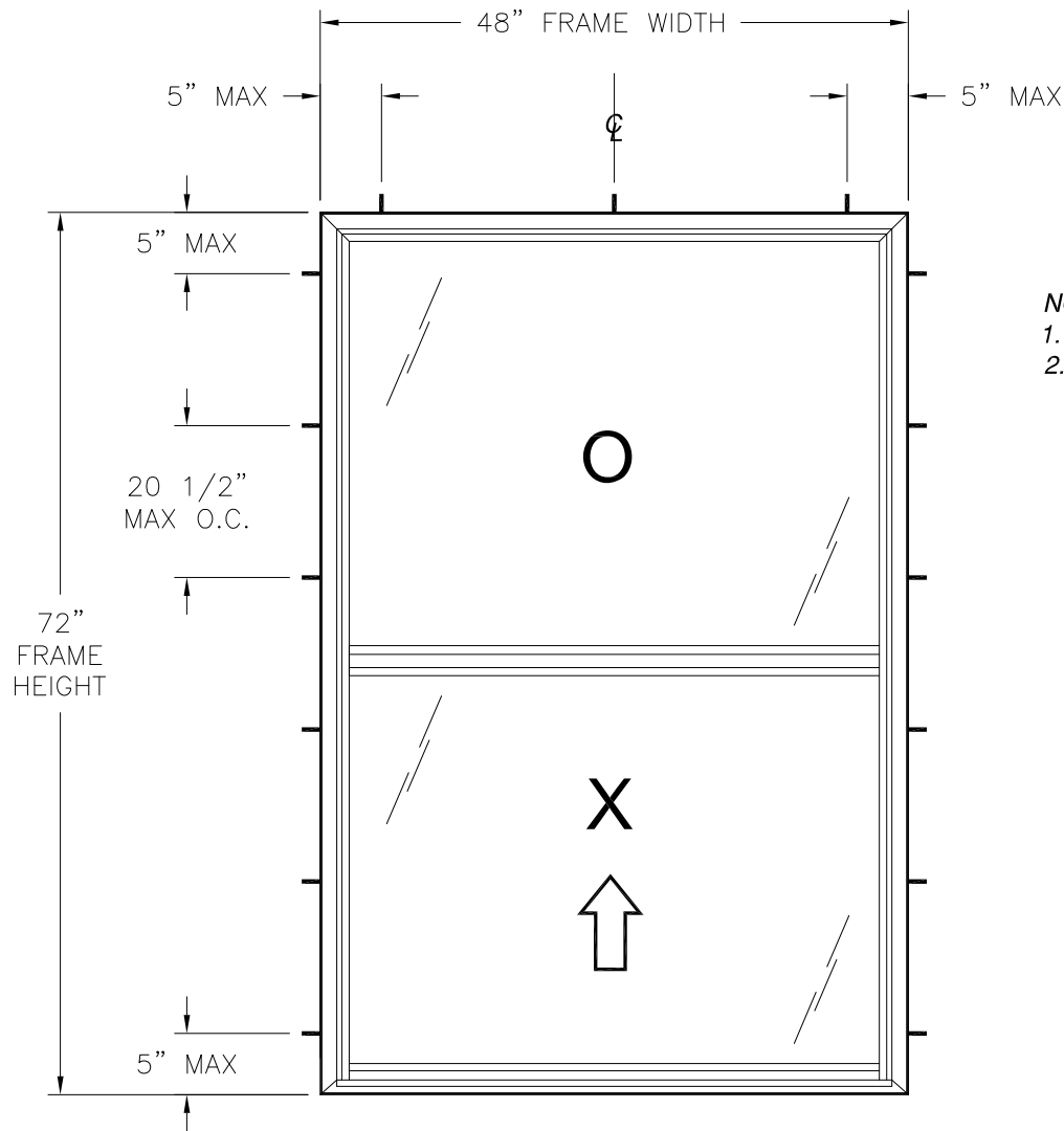
220 VINYL SINGLE HUNG WINDOW EXTERIOR VIEW
